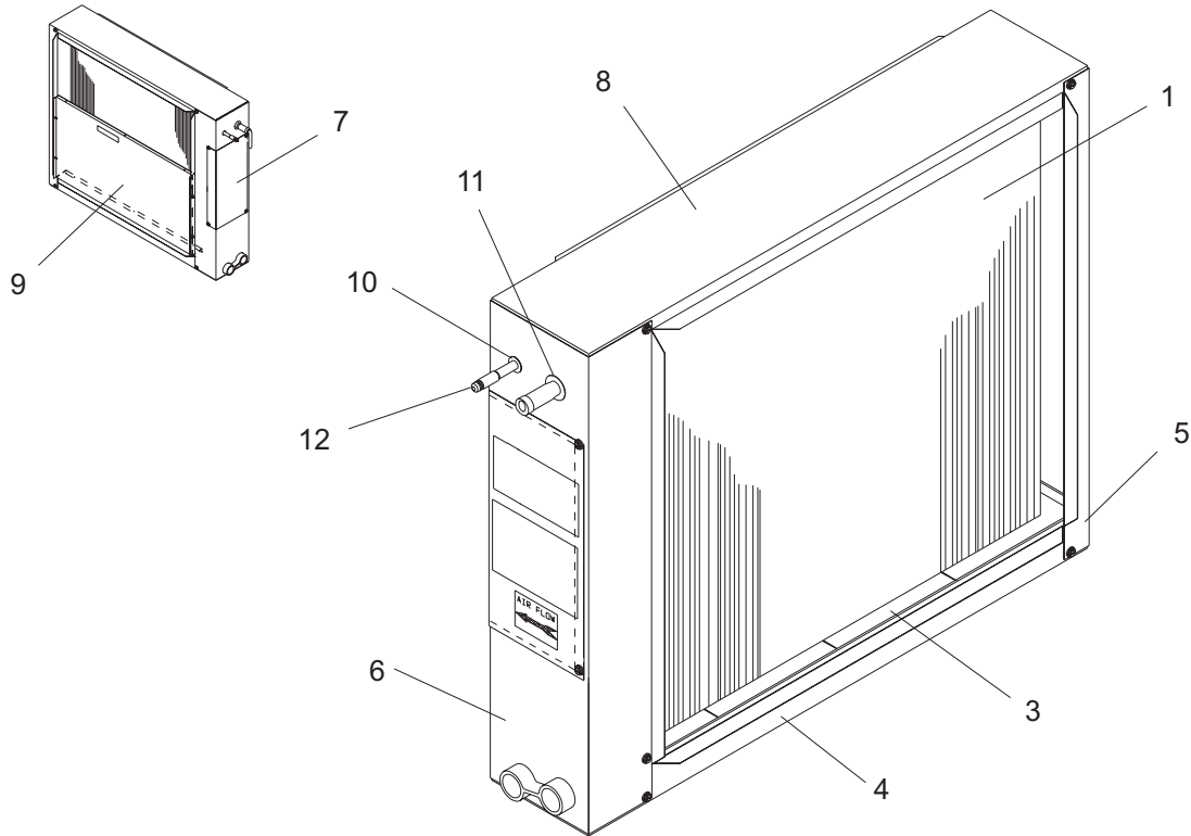
Figure 1 : HORIZONTAL DUCT COILS - R-22 TXV
