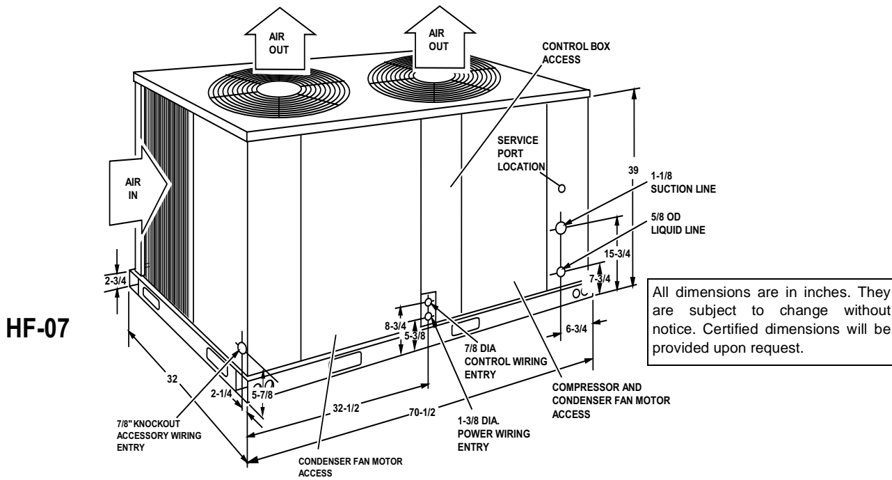
FIGURE 5- UNIT DIMENSIONS & CLEARANCES HF-07
