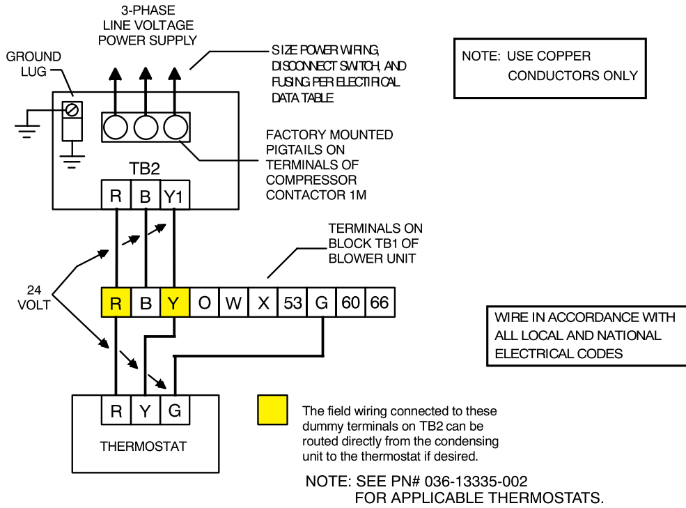
FIGURE 1 - TYPICAL FIELD WIRING WITH AIR HANDLER
