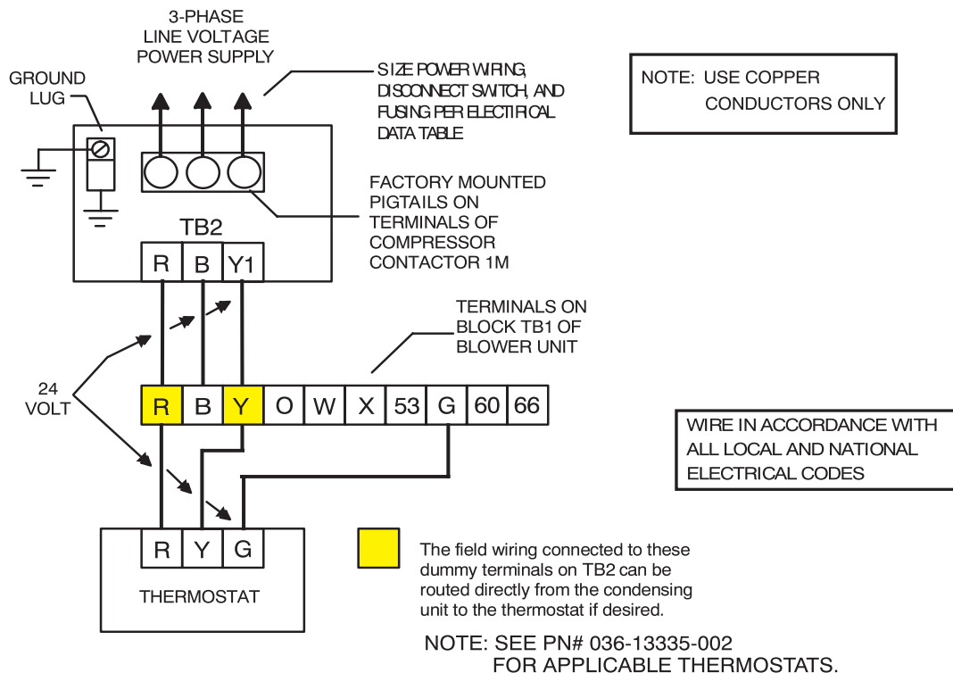
FIGURE 2 - FIELD WIRING - HF-10/LF-10
